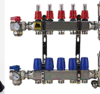
Colector Inox-Open
